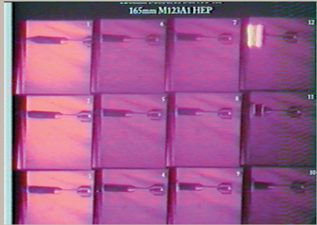
Projectile Penetrates Before Detonating
