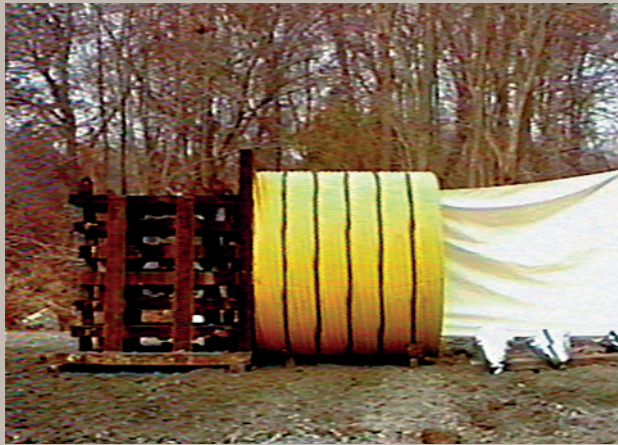
Six Foot Diameter, Reinforced Concrete Cylinder, Confined
